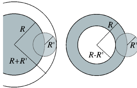
FIG. 1. Illustration of the length scales relevant for the convolution of two spheres. The sphere of radius R (dark gray) is convolved with a sphere of radius R' (light gray) to form a sphere of radius R+R' (white, left) or of radius R-R' (white, right).
