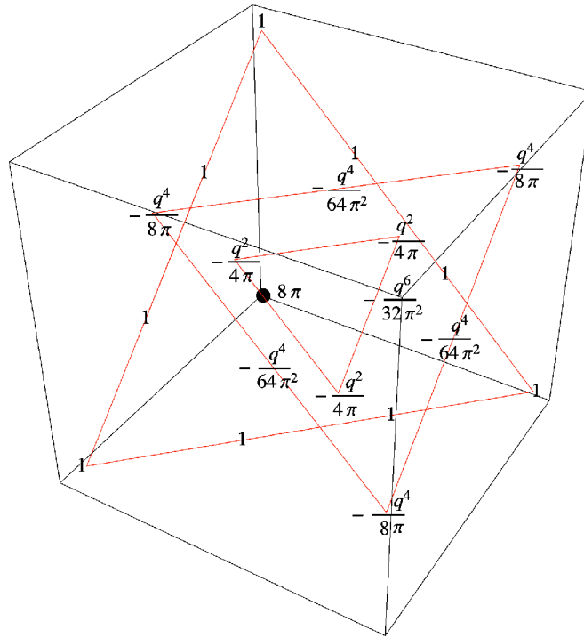
FIG. 2. (Color online) Illustration of \tilde{\mathbf{T}} . The three spatial dimensions correspond to the three indices; the origin (black dot) corresponds to 000. The triangles mark entries with common dimensionalities ( 8\pi lies in the plane spanned by the 1 entries). Note the symmetry under exchange of any two axes and under rotations by 120^\circ around the space diagonal.
